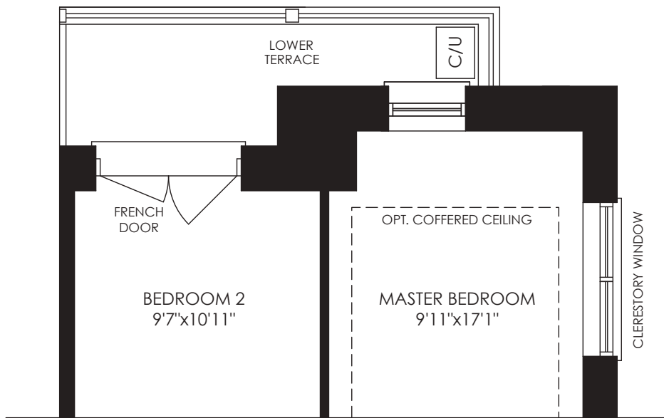
LOWER LEVEL FLOOR PLAN (UNIT 1D) [BLOCK B ONLY] (1389 SQ. FT. - 169 SQ. FT. OUTDOOR)
