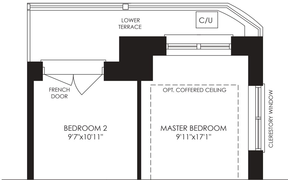
LOWER LEVEL FLOOR PLAN (UNIT 1D) [BLOCK A ONLY] (1399 SQ. FT. - 180 SQ. FT. OUTDOOR)
