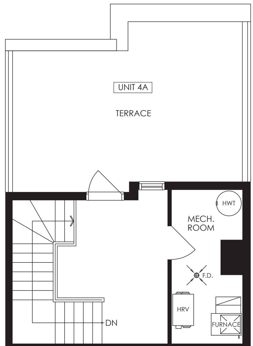
TERRACE FLOOR PLAN (UNITS 4A)
