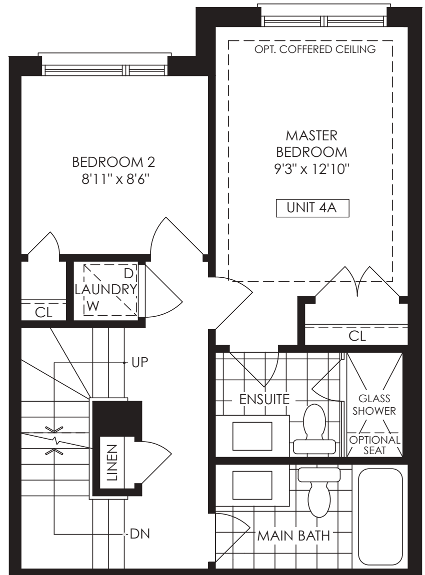
UPPER FLOOR PLAN (UNITS 4A)
