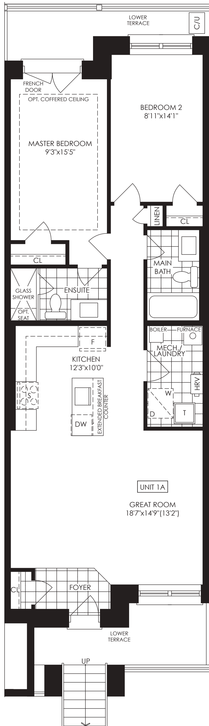
LOWER LEVEL FLOOR PLAN (UNIT 1A)
