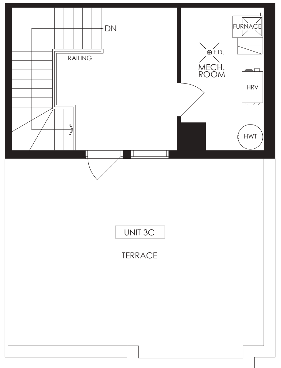
TERRACE FLOOR PLAN (UNIT 3C )
