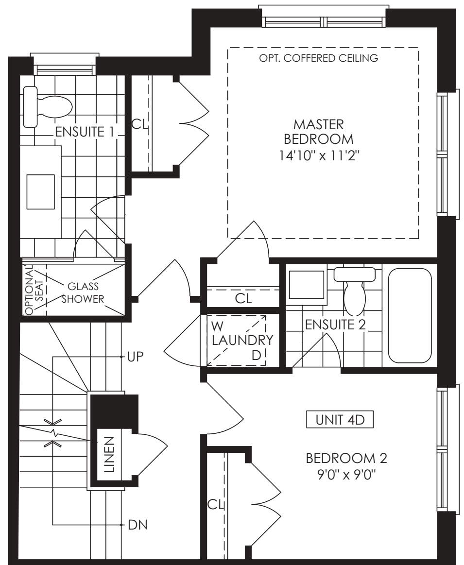
UPPER FLOOR PLAN (UNITS 4D)
