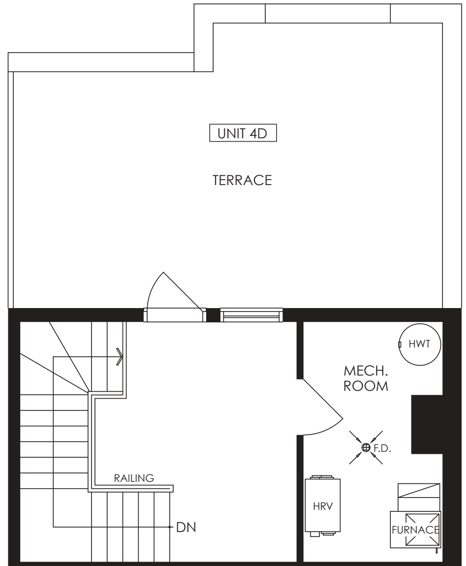
TERRACE FLOOR PLAN (UNITS 4D)
